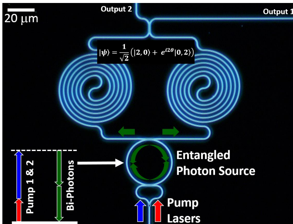
Figure 18. The picture shows a dark-field microscope image of a quantum circuit on the Silicon-On-Insulator chip consisting of an integrated pump splitting circuit, ring resonator ( Q \sim 15k , FSR \sim 5nm ) entangled bi-photon source and Mach-Zehnder analysis circuit. This circuit generates a two-photon path entangled quantum state.
