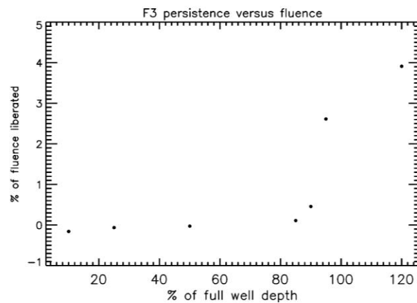
Figure 10. The plot shows the increase in persistence once the exposed fluence is greater than 100% of the full well.
