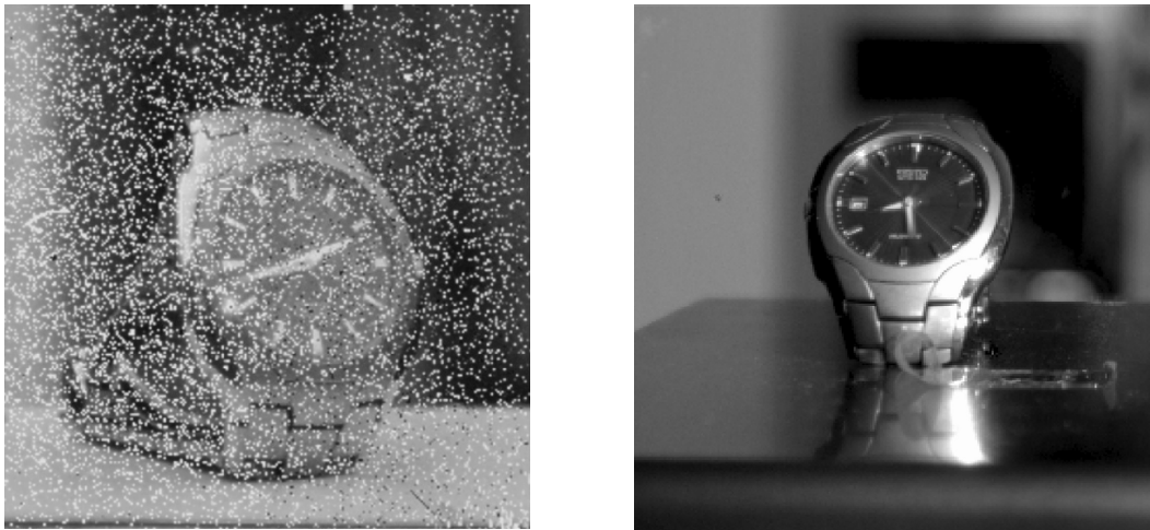
Figure 14. The photos show images of a watch taken with the GM-APD detector arrays developed in this project. The improvement in the image is due to the use of a better bonding process.
