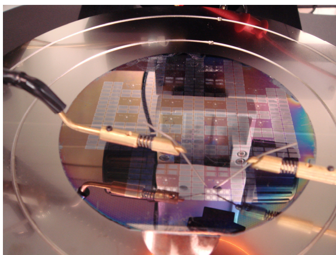
Figure 36. This image is a close-up of a device wafer being tested on the probe station.
