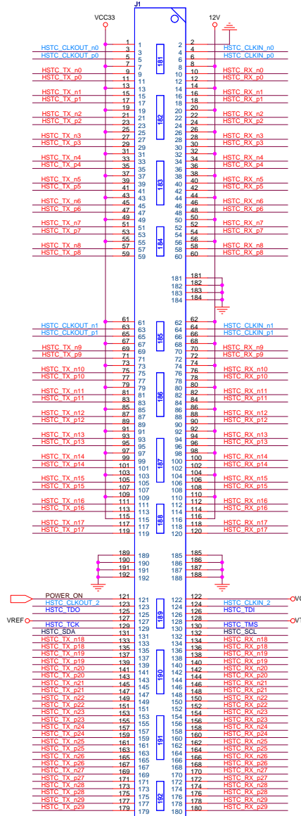
QSH-090-01-F-D-A HSTC Connector - Female (Motherboard Bottom-side) or Daughter Board
