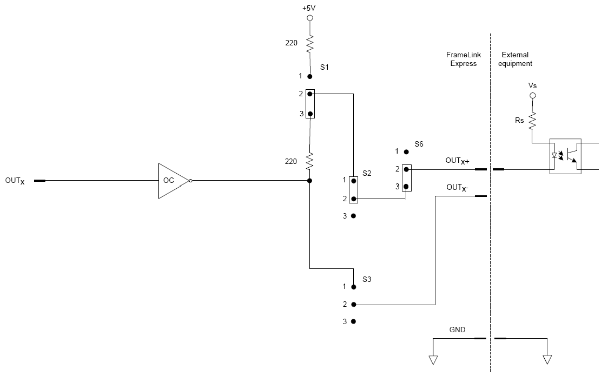
Figure E.8 – Open Collector using Common Ground Output Circuit
