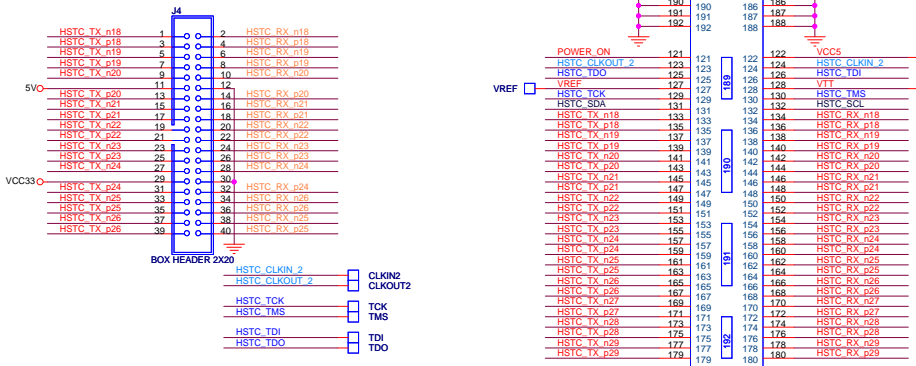
QSH-090-01-F-D-A HSTC Connector - Female (Motherboard Bottom-side) or Daughter Board
